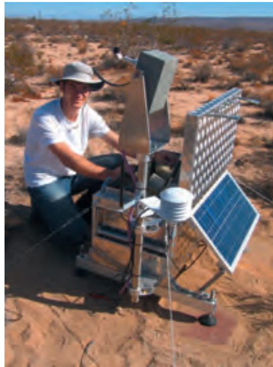
One of Solar Millennium AG's meteorological measuring stations
